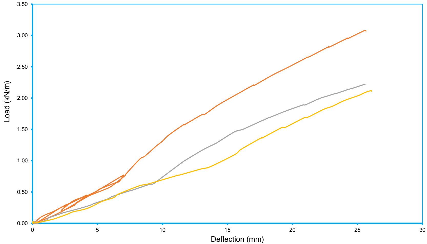
Chart 4 - Uniformly Distributed Line Load for Q-railing EasyGlass Strong Balustrade System Incorporating 25.52 mm PVB Glass Top Mounted into Concrete
