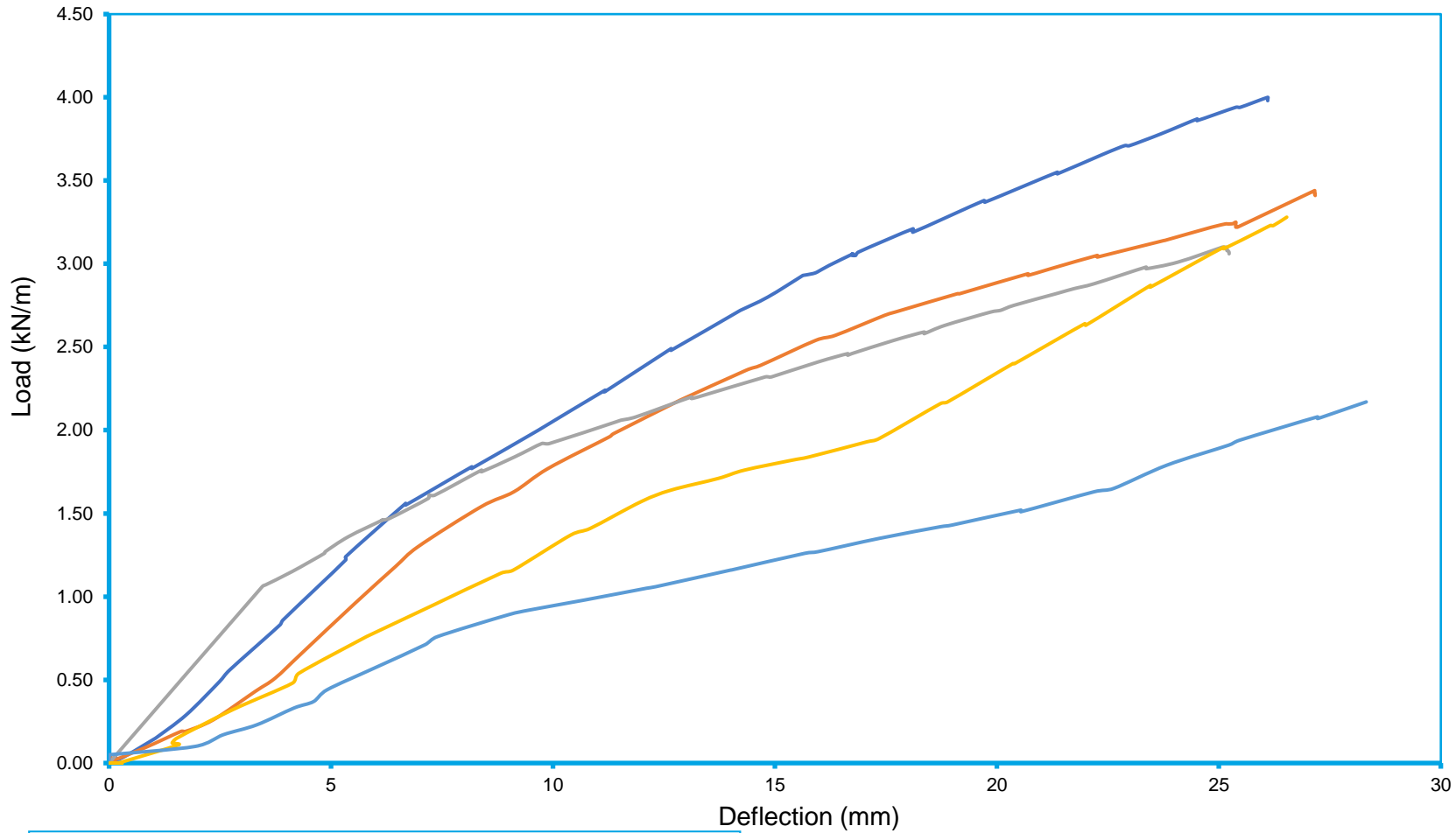
Chart 3 - Uniformly Distributed Line Load for Q-railing EasyGlass Strong Balustrade System Incorporating 31.52 mm PVB Glass Top Mounted into Concrete
