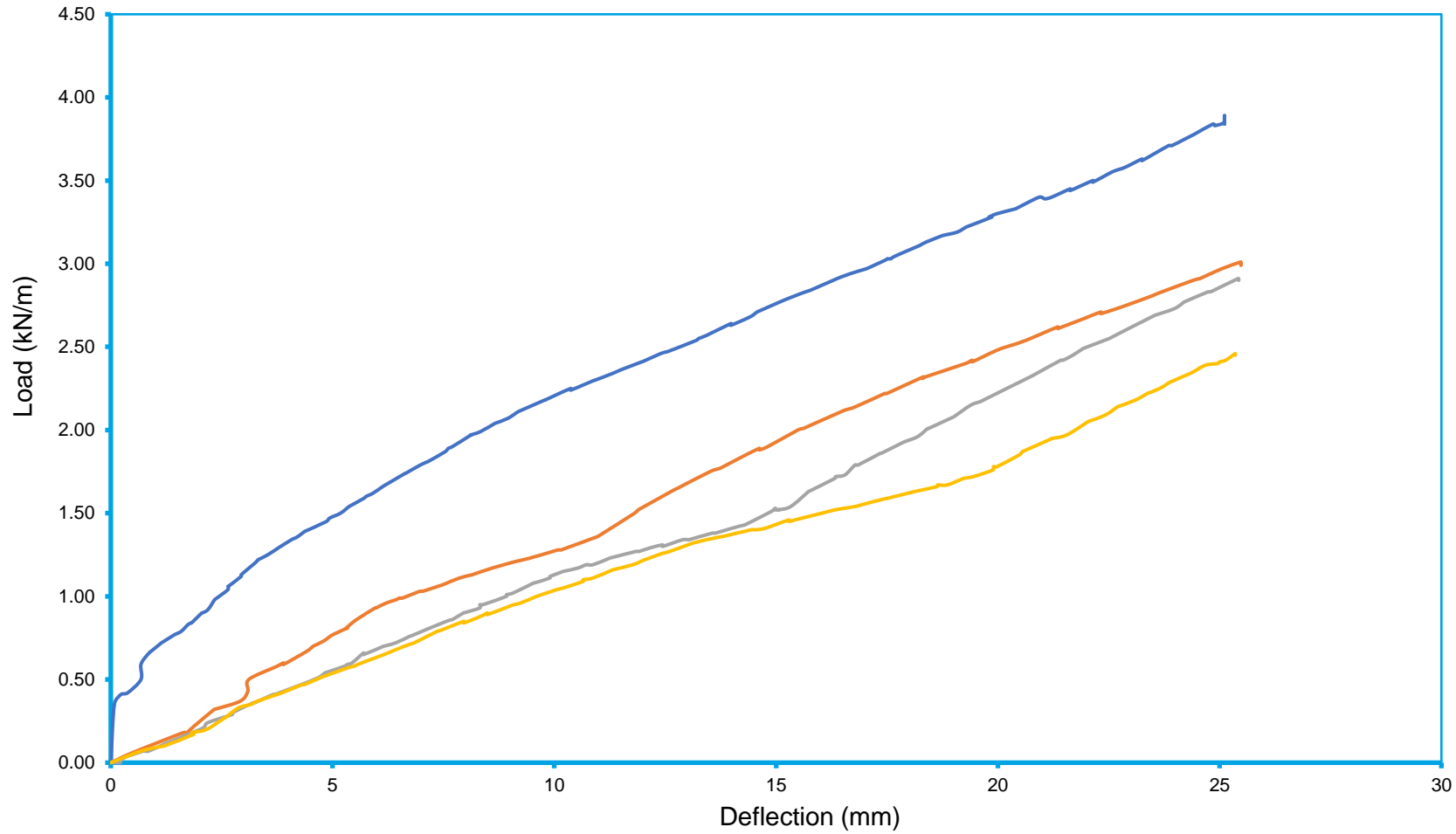
Chart 1 - Uniformly Distributed Line Load for Q-railing EasyGlass Strong Balustrade System Incorporating 31.52 mm Sentry Glass Top Mounted into Concrete
