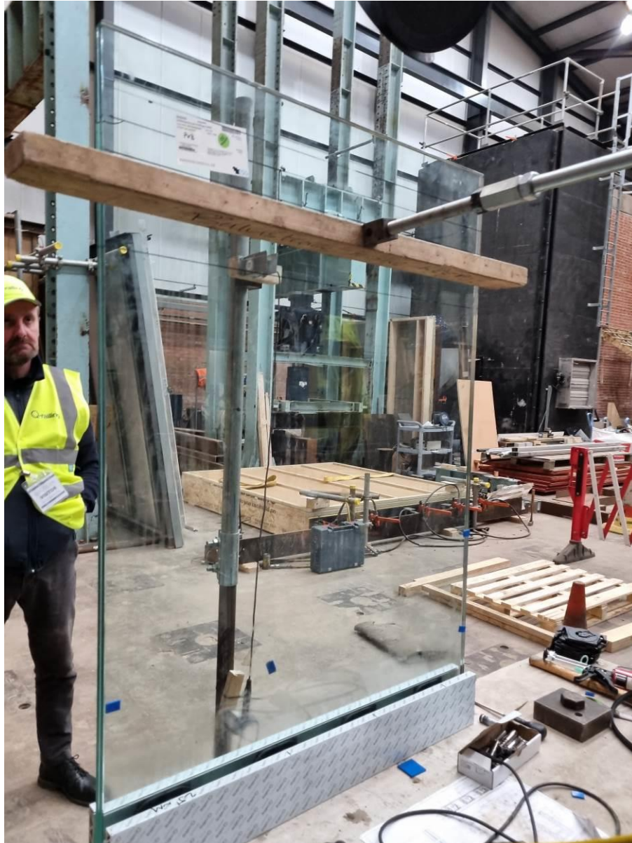
Plate 1 – Generic Test Configuration Uniformly Distributed Line Load
