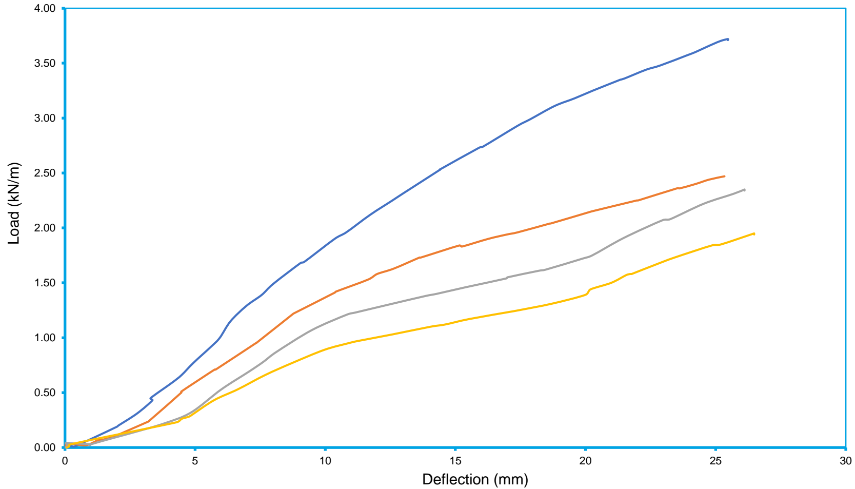
Chart 2 - Uniformly Distributed Line Load for Q-railing EasyGlass Strong Balustrade System Incorporating 25.52 mm Sentry Glass Top Mounted into Concrete
